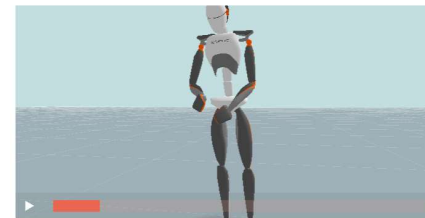
REBA outcome
